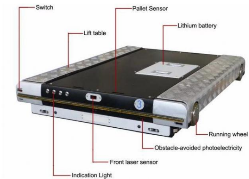
Radio Shuttle 2G-Standard Configuration
